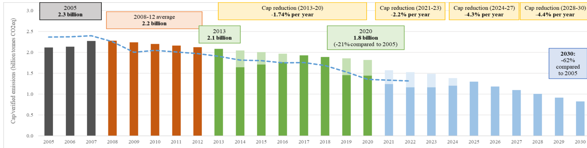
Figure 2: Emissions cap in the EU ETS compared with verified emissions (considering the 2023 revision of the ETS Directive, i.e. rebasing in 2024 and 2026, including the maritime transport sector in 2024 and the linear reduction factor of 4.3% in 2024-2027 and 4.4% from 2028). Aviation is not included. Due to changes in scope, the 2005-2007 figures are not directly comparable with the latest ones. From 2021, the EU ETS no longer covers installations in the UK, only electricity generators in Northern Ireland. Legend: bars (cap), light shaded bars in 2014-2016 (allowances backloaded from auctions), light shaded bars from 2019 (feeds of allowances to the Market Stability Reserve), dashed line (verified emissions).
